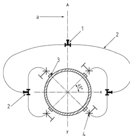
Figure 3 Example of slit type of pressure tapping with ring chamber, suitable for small/medium diameter test sections
