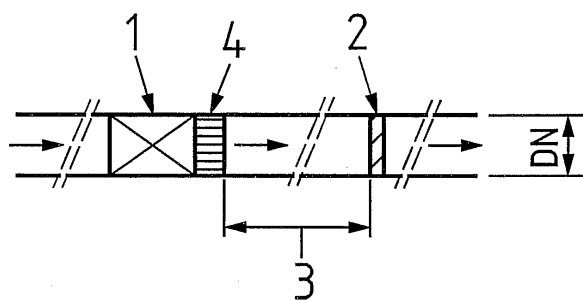
Test 2A: with a straightener
