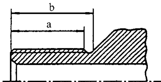
Figure B.2 - Thread
