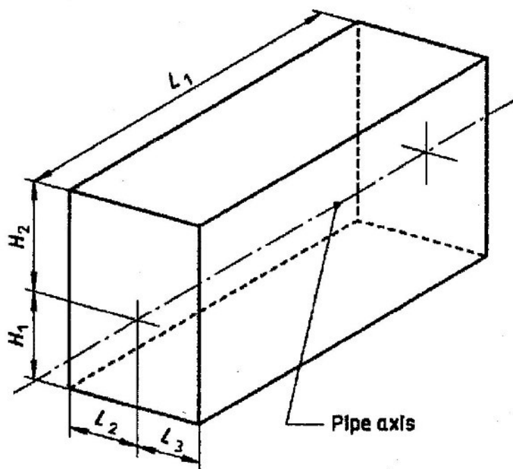
Figure B.1 – Meter size and overall dimension
