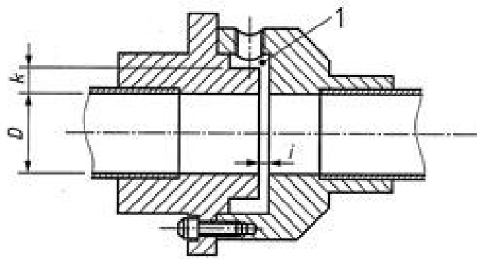
Figure 3 Example of slit type of pressure tapping with ring chamber, suitable for small/medium diameter test sections
