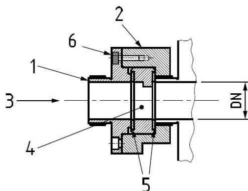
Figure A.1 Threaded type disturbance generator – Arrangement of swirl generator units
