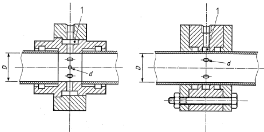
Figure 1 Pressure loss test: layout of measuring section
