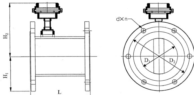
Figure C.1 The flange dimension of Vortex water meters
