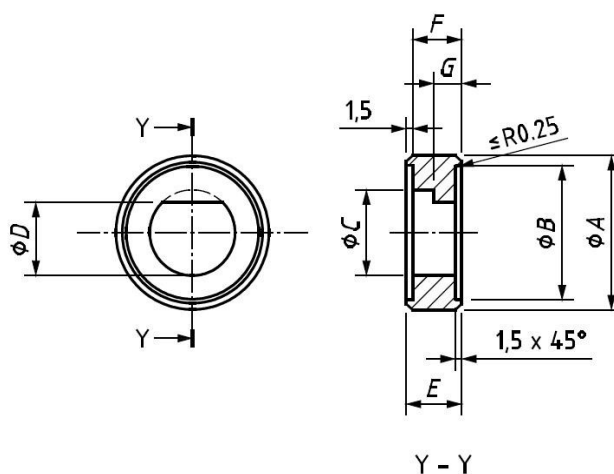
Figure A.6 Flow disturber for a threaded type disturbance generator
