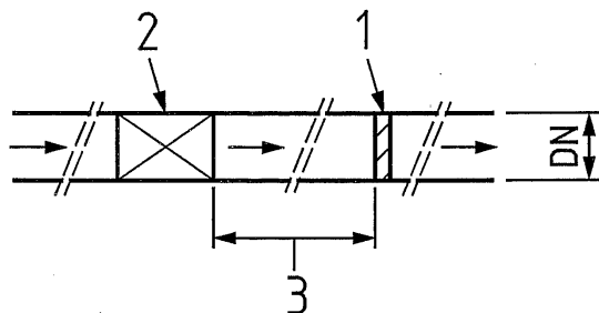
Test 1A: with a straightener
