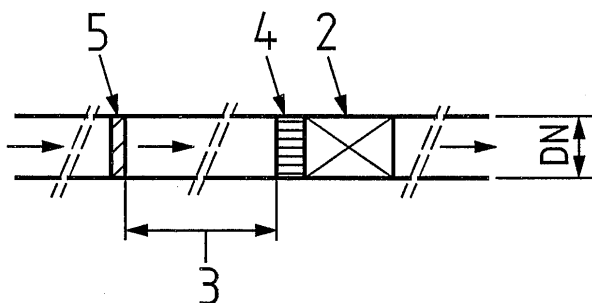
Test 3A: with a straightener
