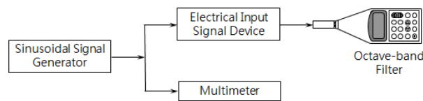
Figure 3 Test system for relative attenuation of filter
