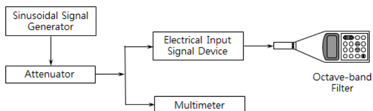
Figure 2 Test system for level linearity of filter
