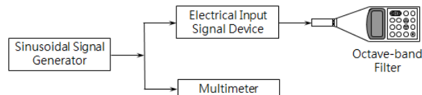
Figure 1 Test system for flat frequency response of octave-band-filter
