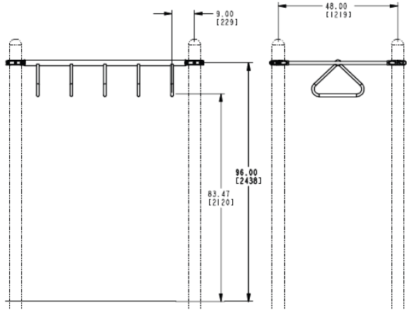
Elevation Views
